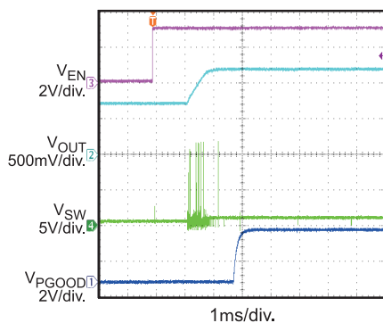
Pre-Bias Start-Up
